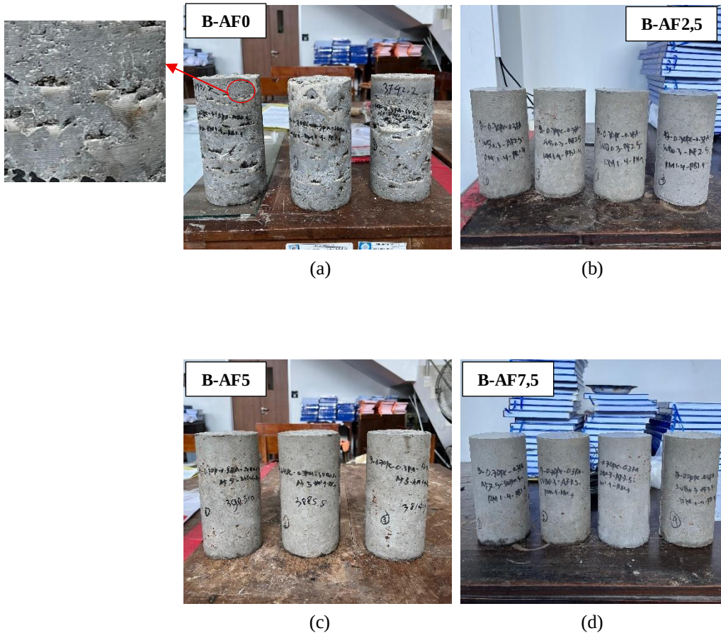
Figure 3. The condition of the concrete after 24 hours of curing (a) concrete without alkali activator; (b) concrete with 2.5% alkali activator; (c) concrete with 5% alkali activator; (d) concrete with 7.5% alkali activator.
