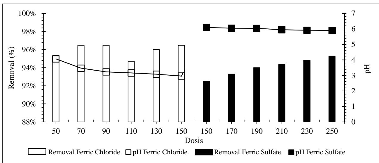
Gambar 1 Hasil Koagulasi-Flokulasi Ferric sulfate ( \text{Fe}_2(\text{SO}_4)_3 ) dan Ferric chloride ( \text{FeCl}_3 \cdot 6\text{H}_2\text{O} )
